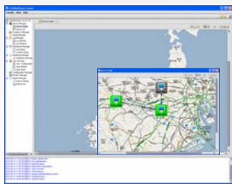
Device Manager
